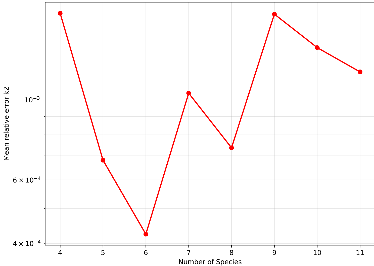
50, 50 — Mean relative error k2 vs number of species (zoomed: 4 to 11 species)
